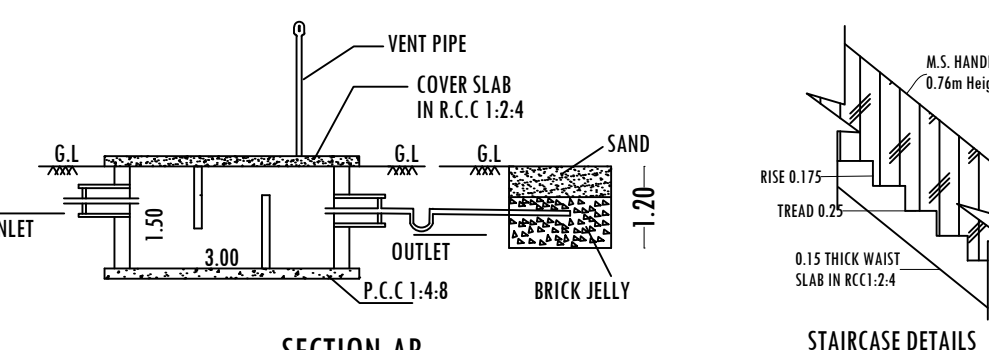
SECTION-AB
