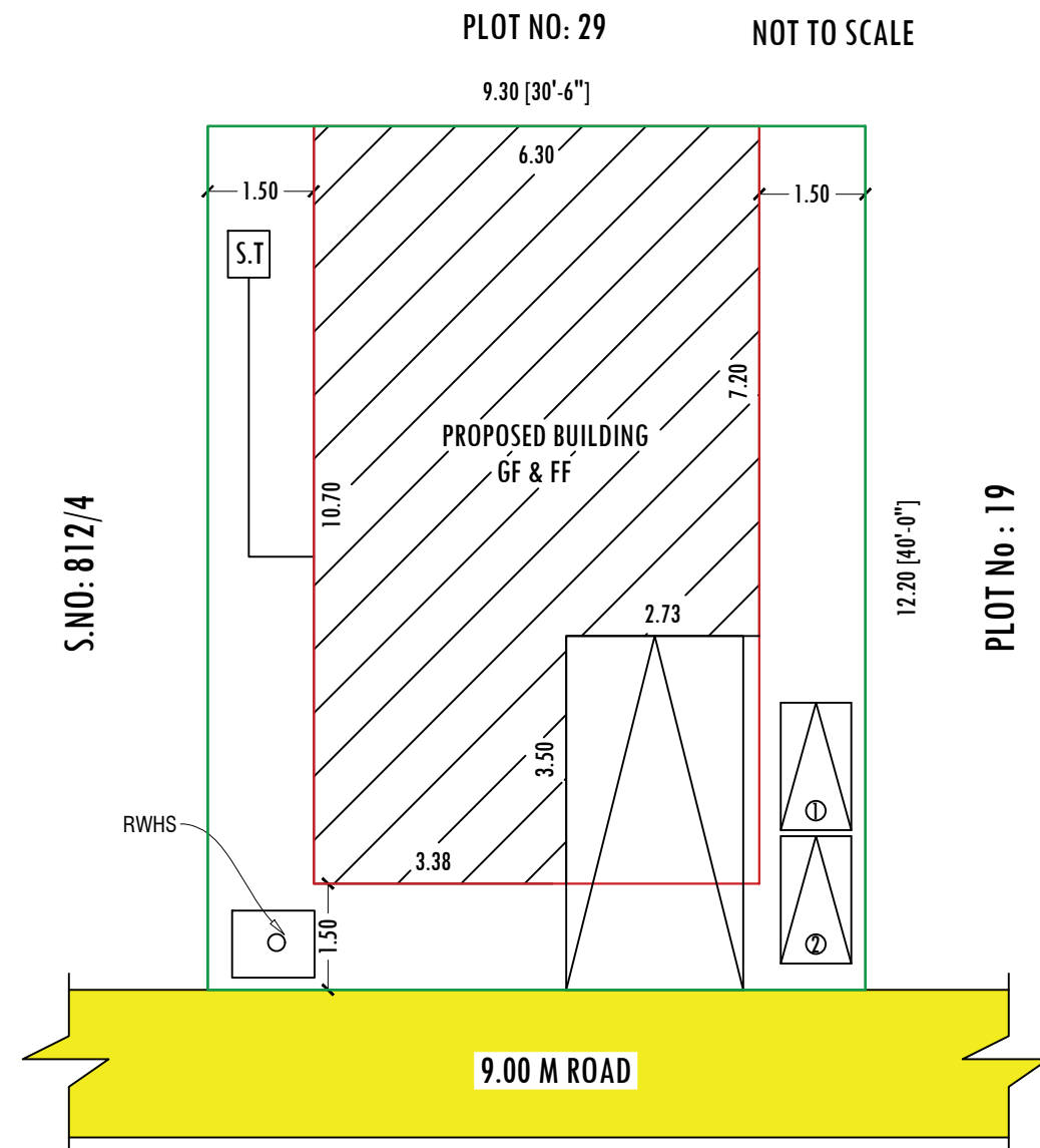
SITE PLAN
