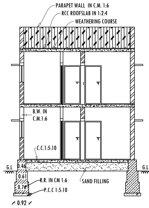
SECTION -AA
