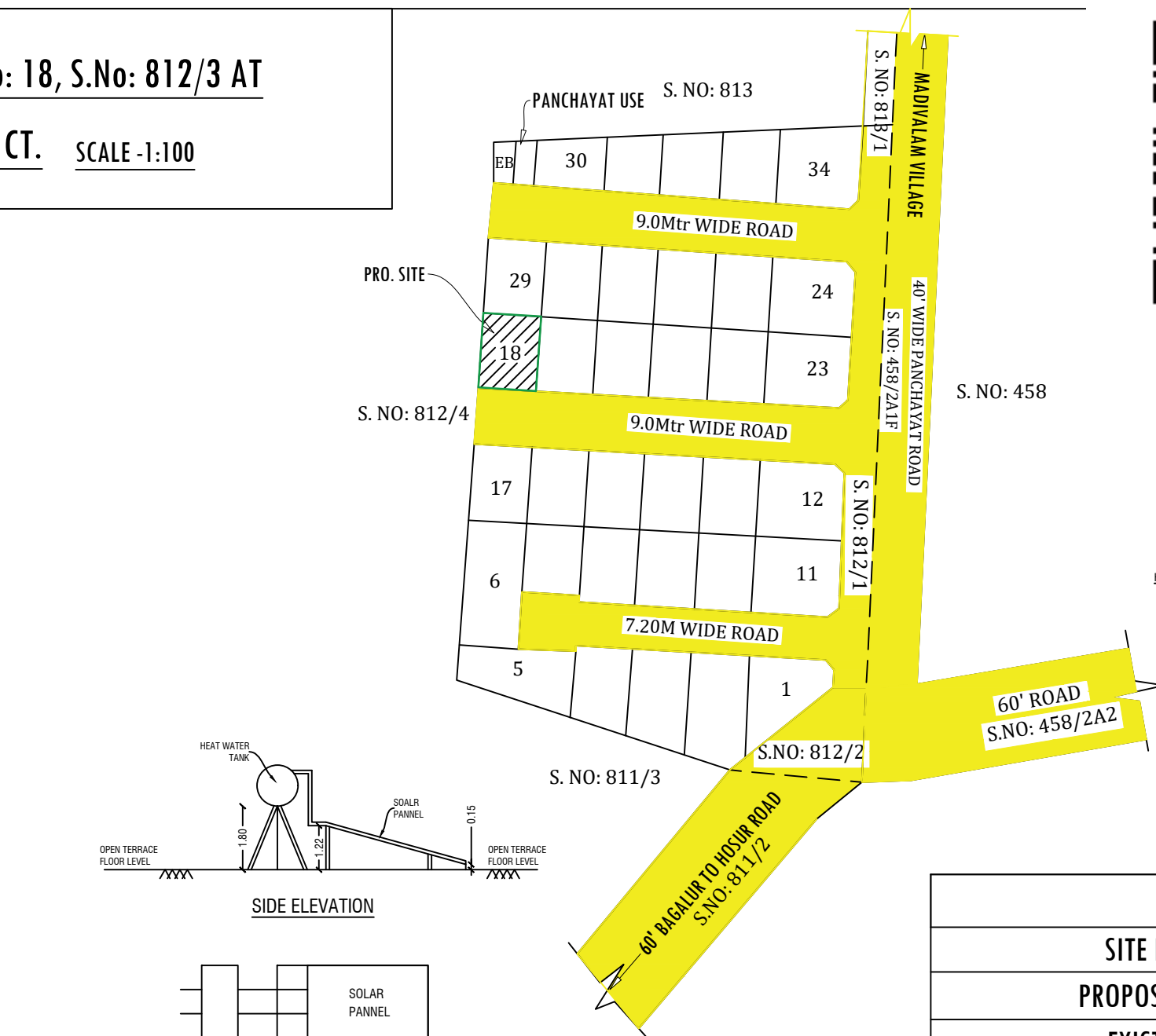
LOCATION PLAN
