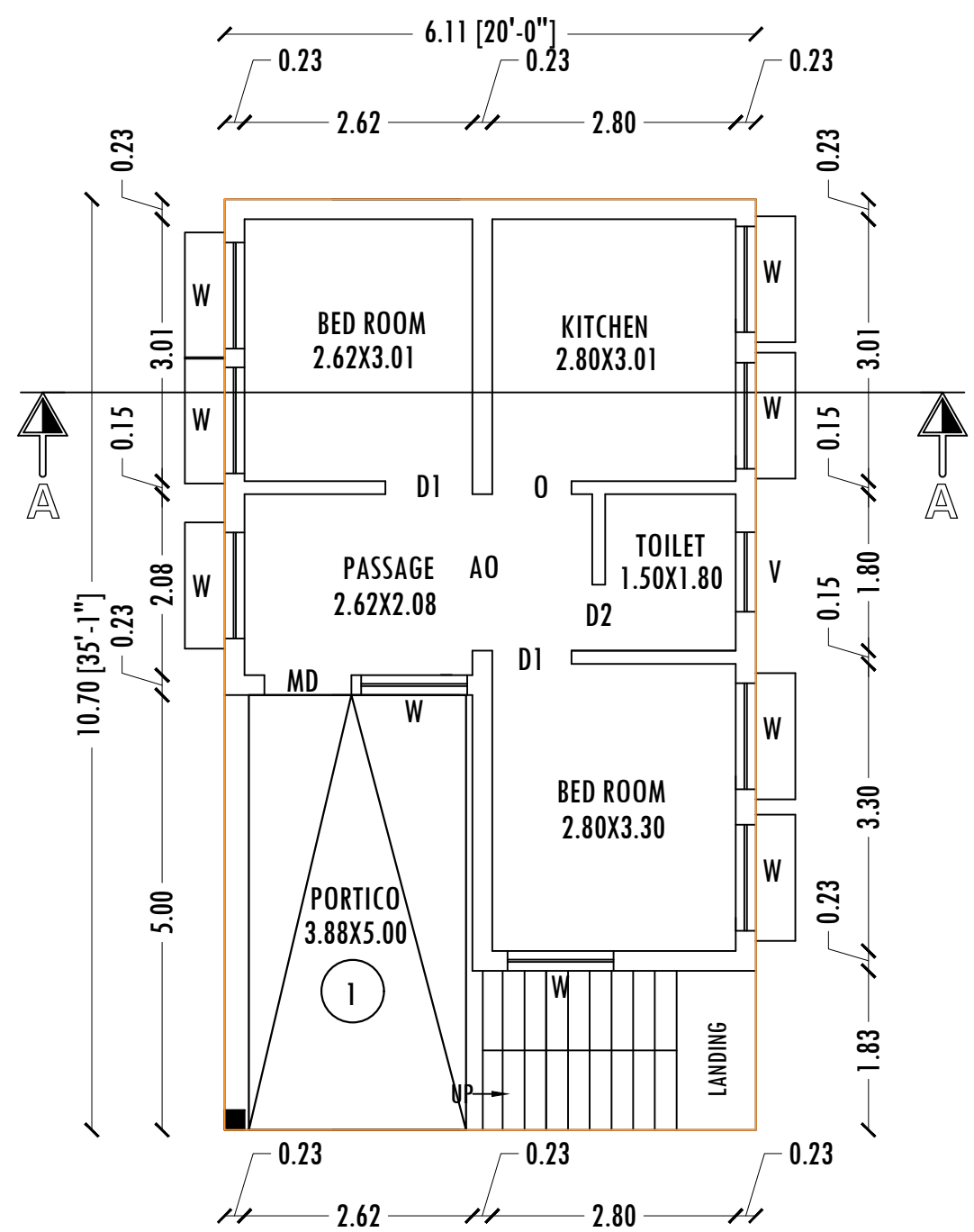
EXTG-GROUND FLOOR PLAN
