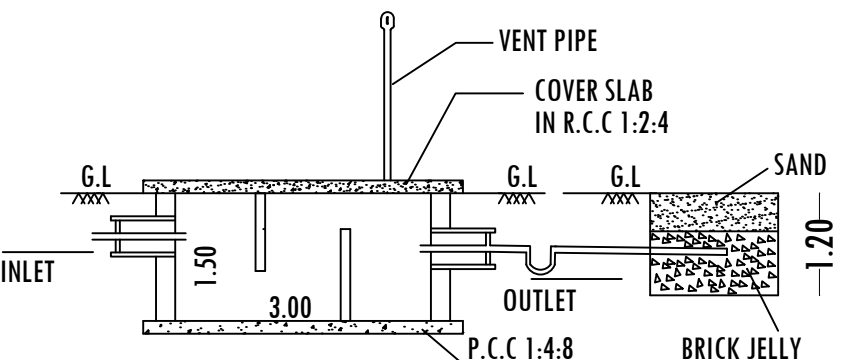
SECTION-AB
