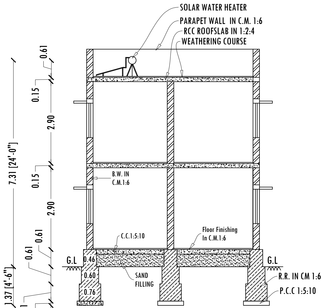
SECTION-AA
