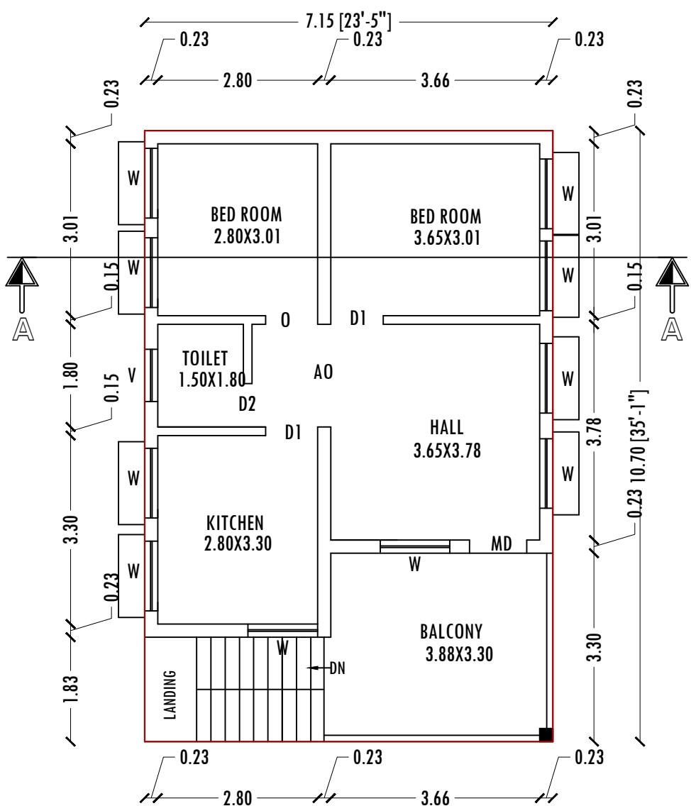
PRO-SECOND FLOOR PLAN
