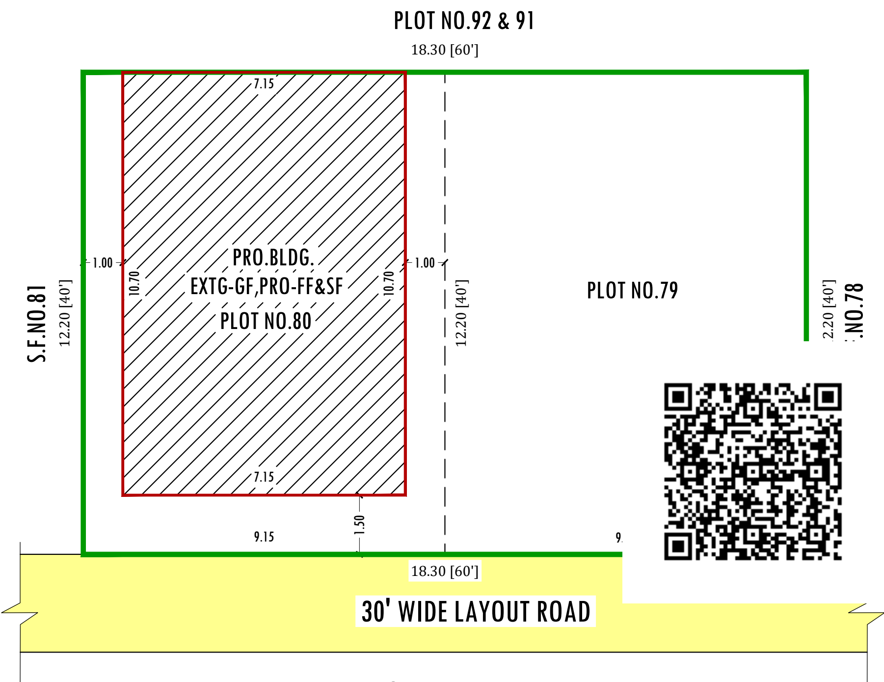
SITE PLAN
