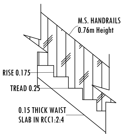
STAIRCASE DETAILS
