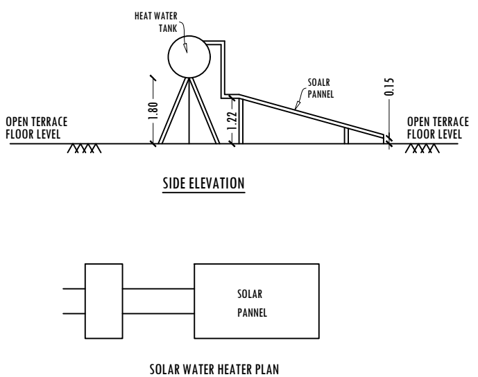
SOLAR WATER HEATER PLAN
