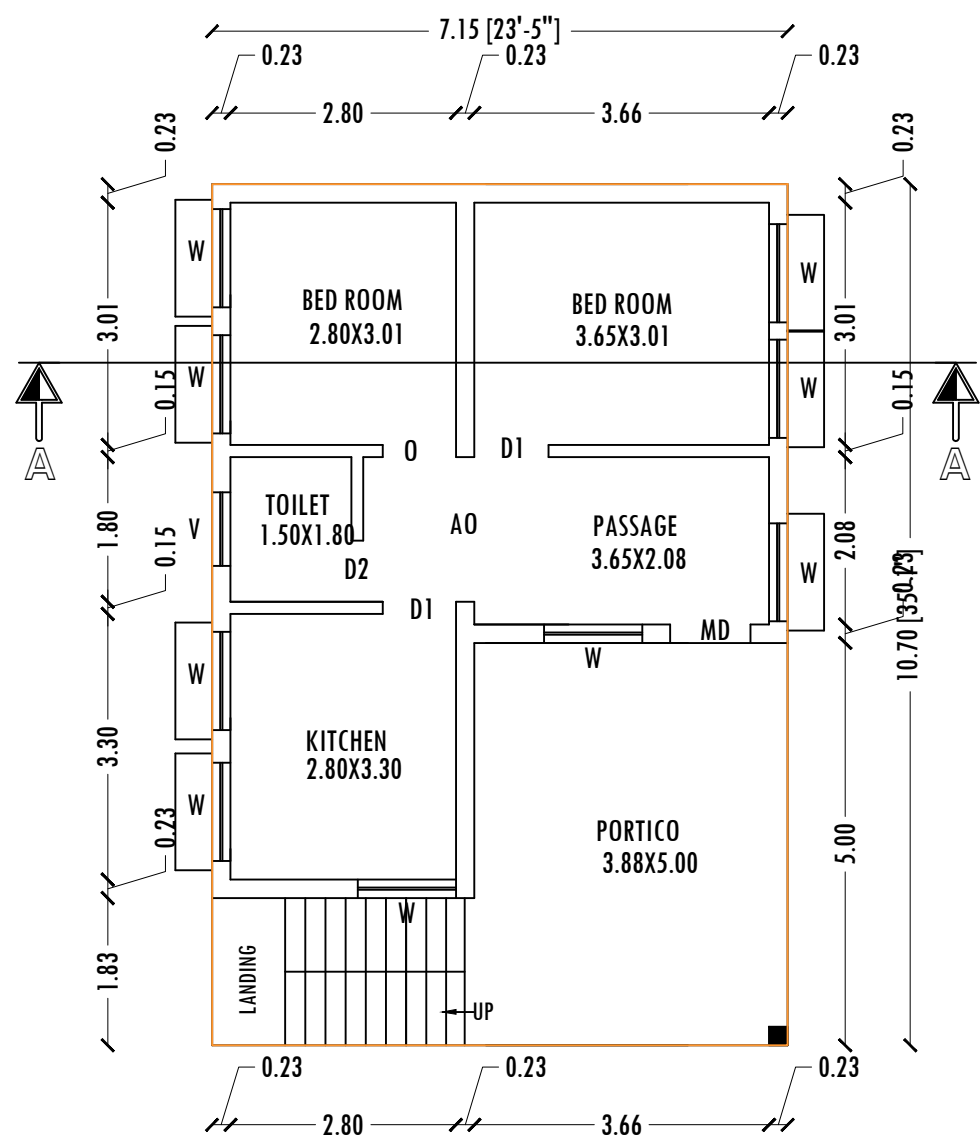
EXTG-GROUND FLOOR PLAN
