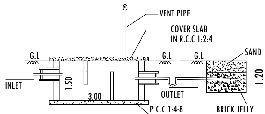
SECTION-AB
