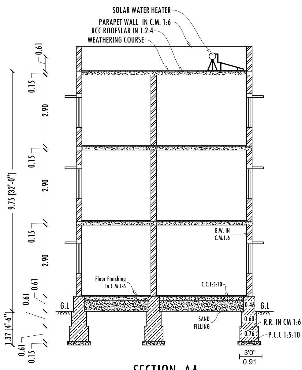
SECTION -AA
