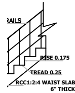
TAIRCASE DETAILS SCALE- 1:20
