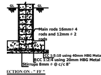
SECTION ON - "FF"
