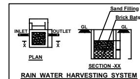
RAIN WATER HARVESTING SYSTEM
