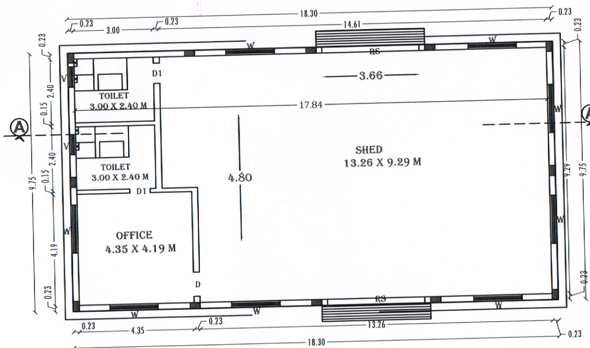
SHED- GROUND FLOOR PLAN
