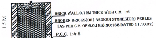
SECTION OF RAIN WATER PERCOLATION BED
