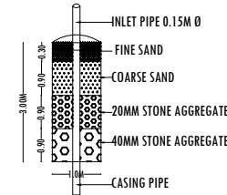
DETAILS OF RAIN WATER HARVESTING STRUCTURES
