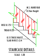
STAIRCASE DETAILS SCALE- 1:20
