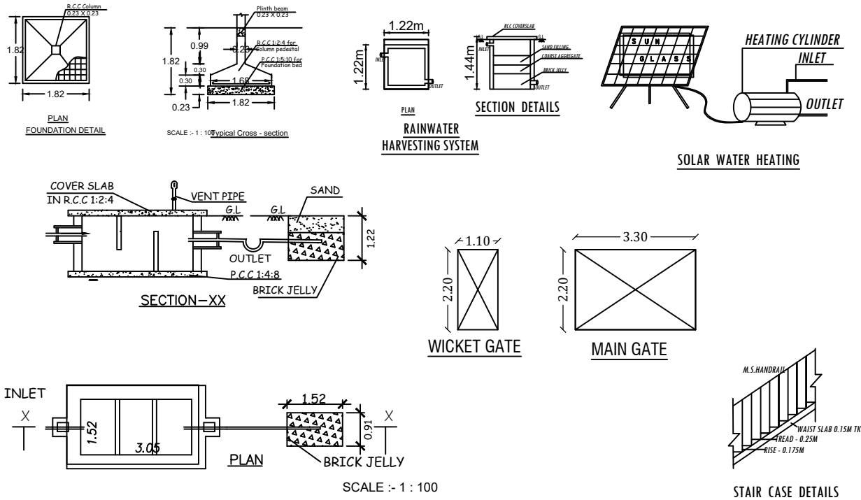
SEPTIC TANK & DISPERSION TRENCH DETAILS
