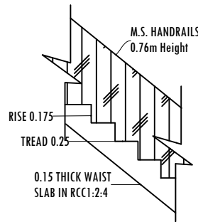
STAIRCASE DETAILS
