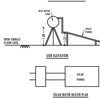
SOLAR WATER HEATER PLAN
