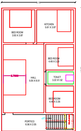
PRO. GROUND FLOOR PLAN.
