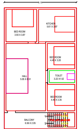
PRO. FIRST FLOOR PLAN.
