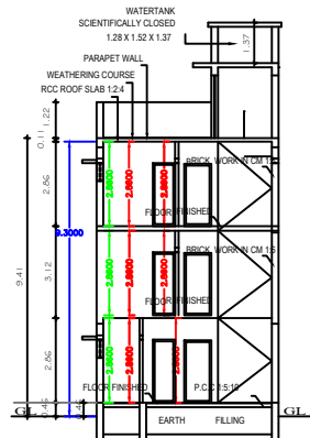
SECTION "A-B"
