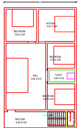
PRO. SECOND FLOOR PLAN.
