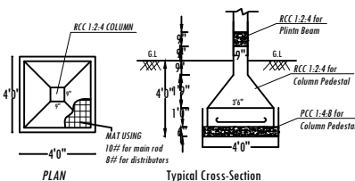
Typical Cross-Section
