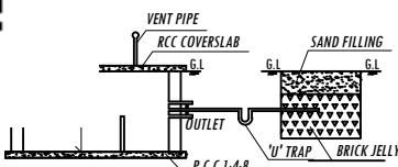
SECTION DETAILS
