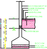
FOUNDATION DETAILS SCALE (1" = 4'0" 1:50)
