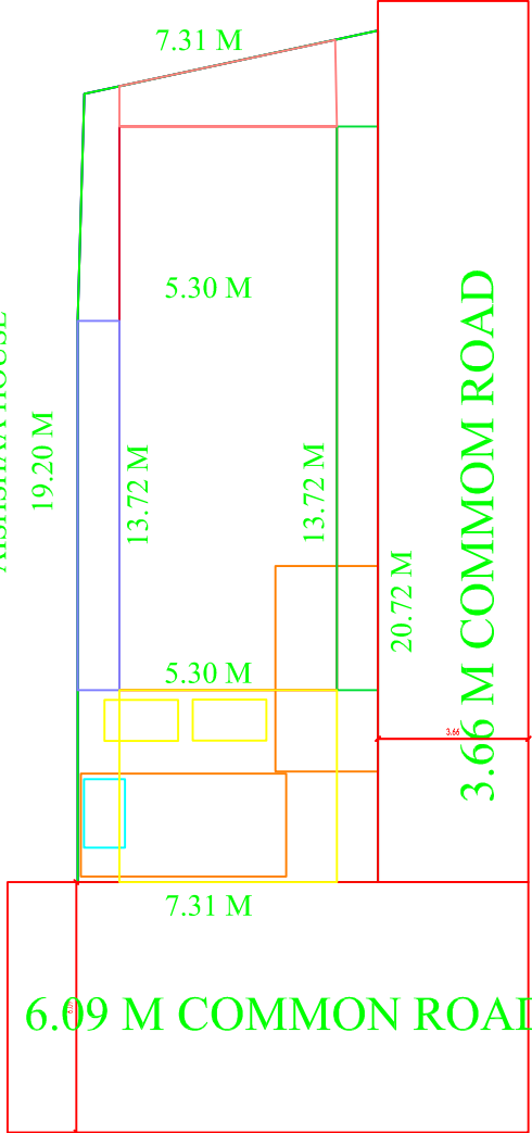
SITE PLAN
