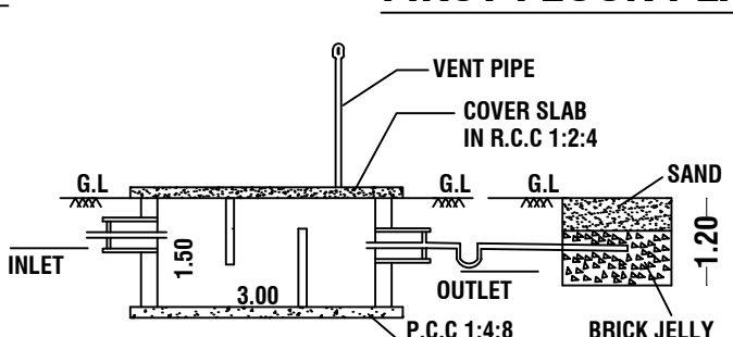
SECTION-AB
