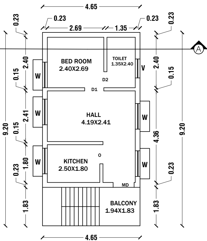
SECOUND FLOOR PLAN
