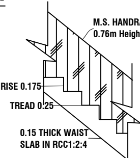
STAIRCASE DETAILS
