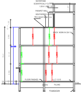
SECTION "A-B"
