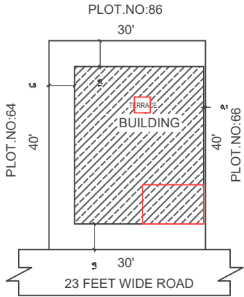
SITE PLAN
