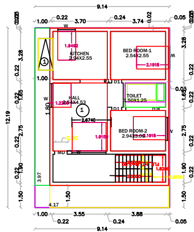
PRO.GROUND FLOOR PLAN SCALE:1:100
