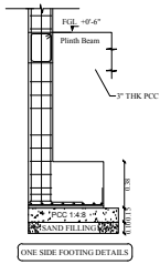
ONE SIDE FOOTING DETAILS
