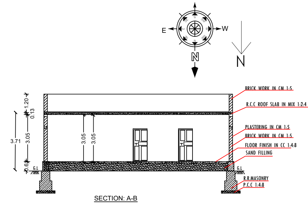
SECTION: A-B
