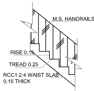
STAIRCASE DETAILS
