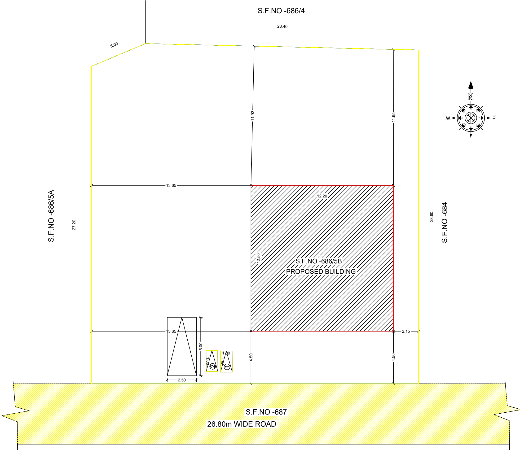
SITE PLAN
