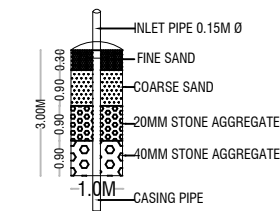
DETAILS OF RAIN WATER HARVESTING STRUCTURES
