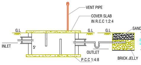
SECTION-AB
