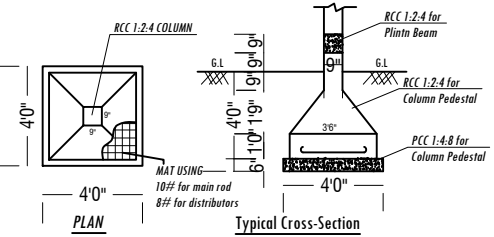
FOOTING DETAILS
