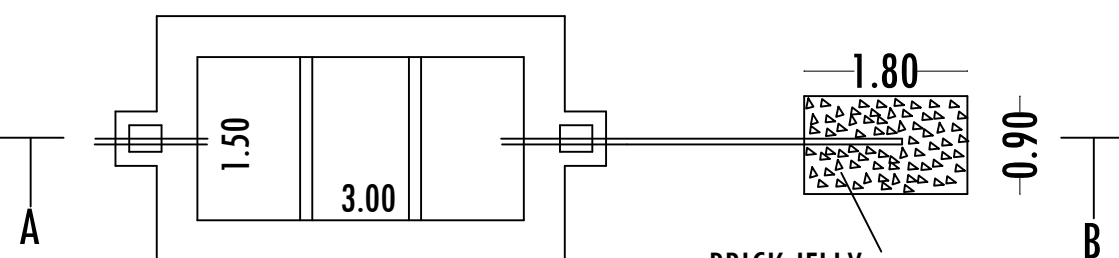
SEPTIC TANK & DISPERSION TRENCH DETAILS
