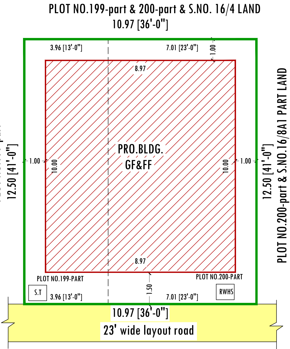
SITE PLAN
