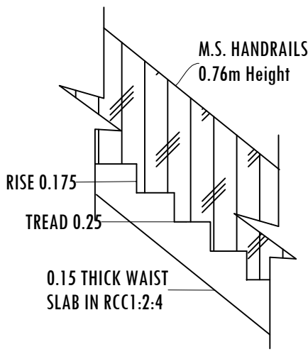
STAIRCASE DETAILS
