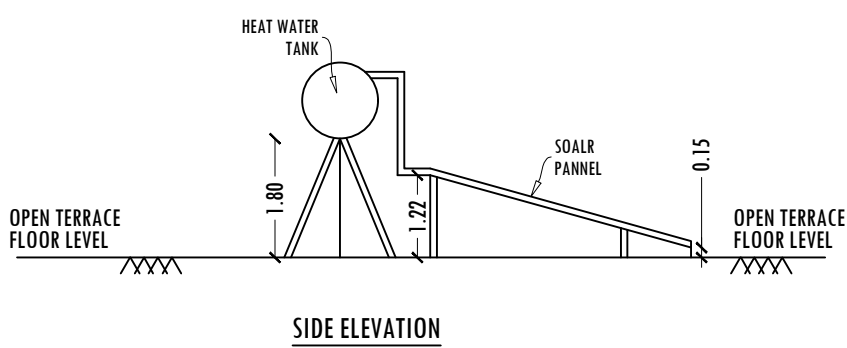
SIDE ELEVATION
