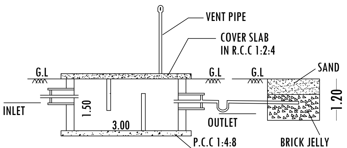
SECTION-AB
