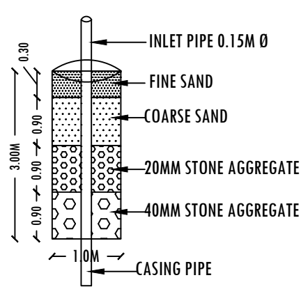
DETAILS OF RAIN WATER HARVESTING STRUCTURES
