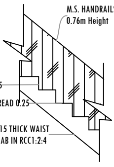
STAIRCASE DETAILS
