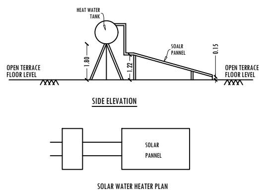
SOLAR WATER HEATER PLAN
