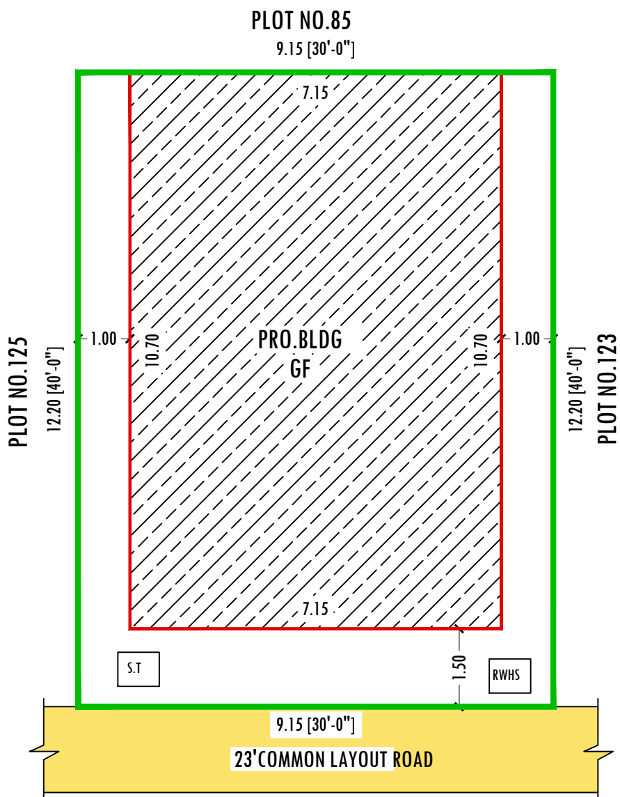
SITE PLAN
