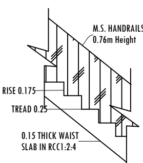
STAIRCASE DETAILS SCALE- 1:20
