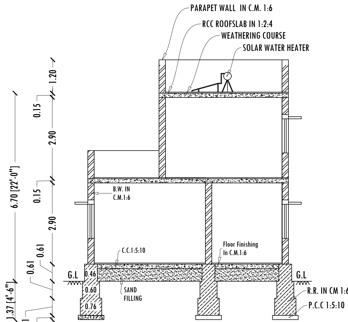
SECTION-AA
