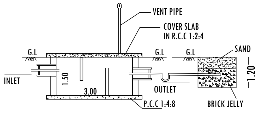
SECTION-AB
