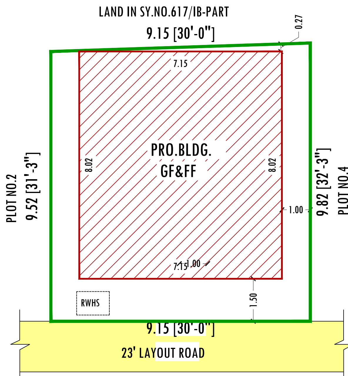
SITE PLAN
