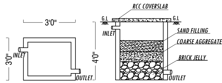
RAINWATER HARVESTING SYSTEM
