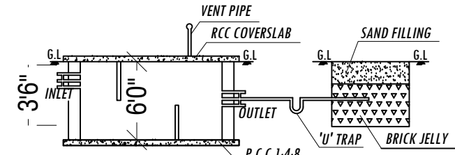
SECTION DETAILS
