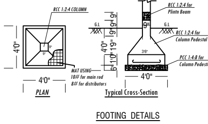
FOOTING DETAILS
