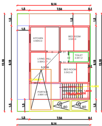
EXI. GROUND FLOOR PLAN SCALE: 1:100
