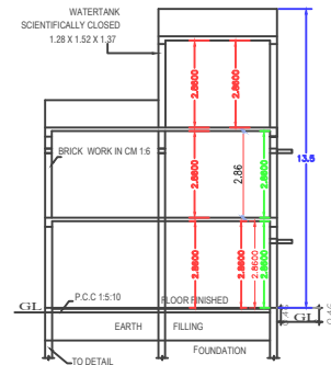
SECTION "A-B"
