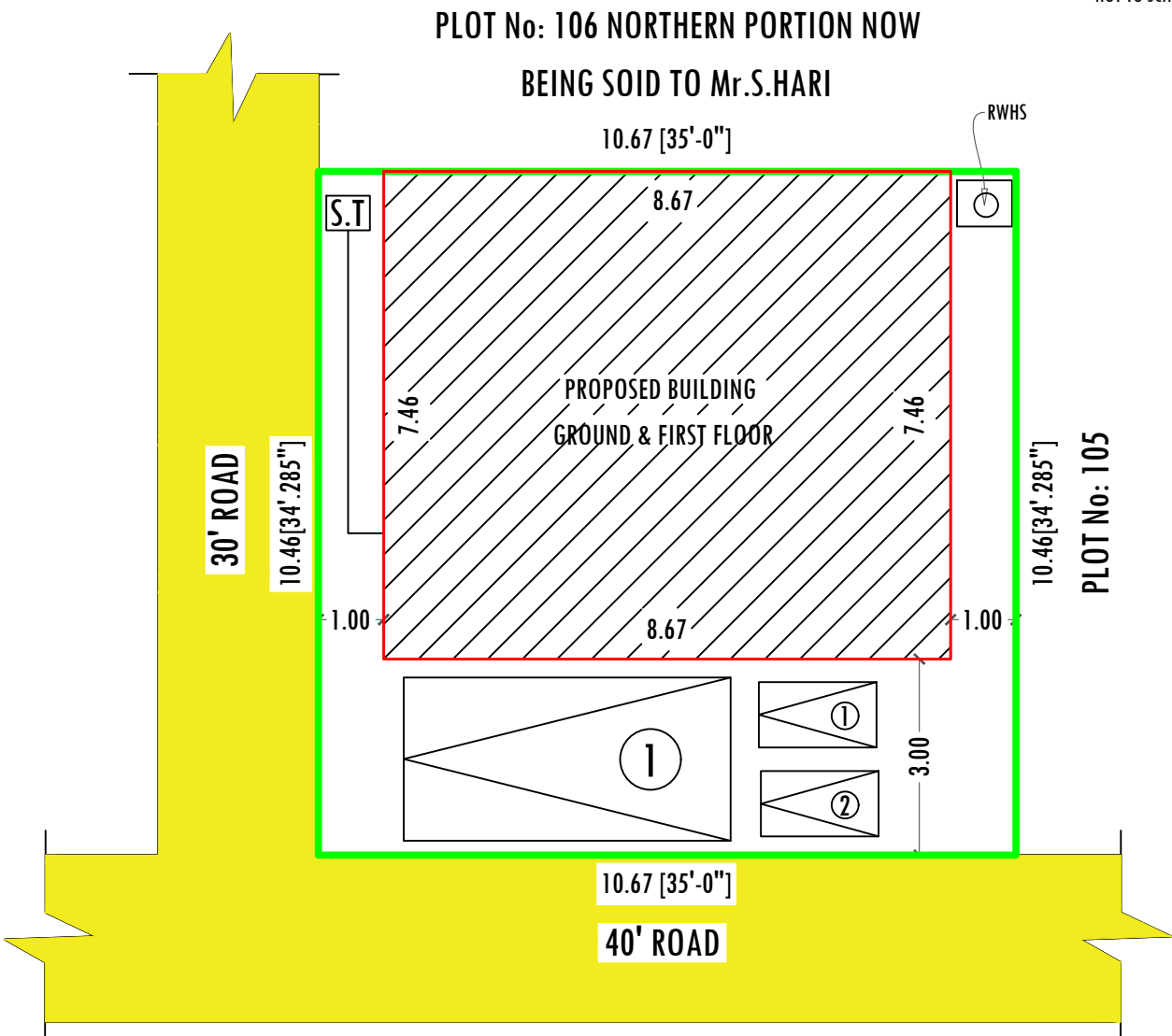
SITE PLAN
