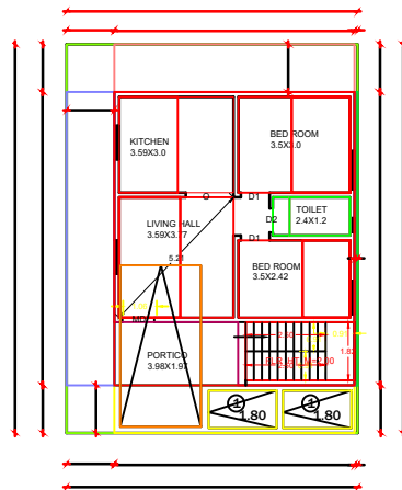
EXI. GROUND FLOOR PLAN SCALE: 1:100
