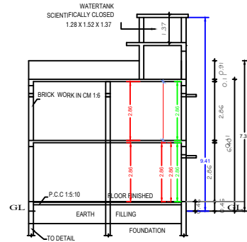
SECTION "A-B"
