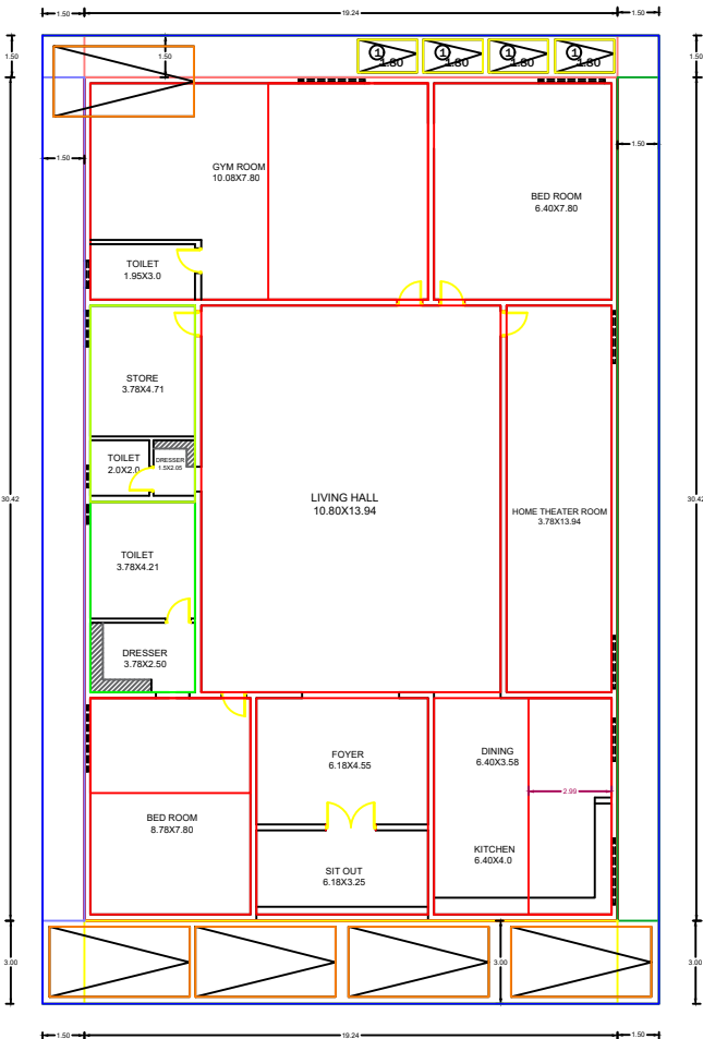
PRO.GROUND FLOOR PLAN SCALE:1:100
