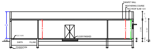
SECTION "A-B"
