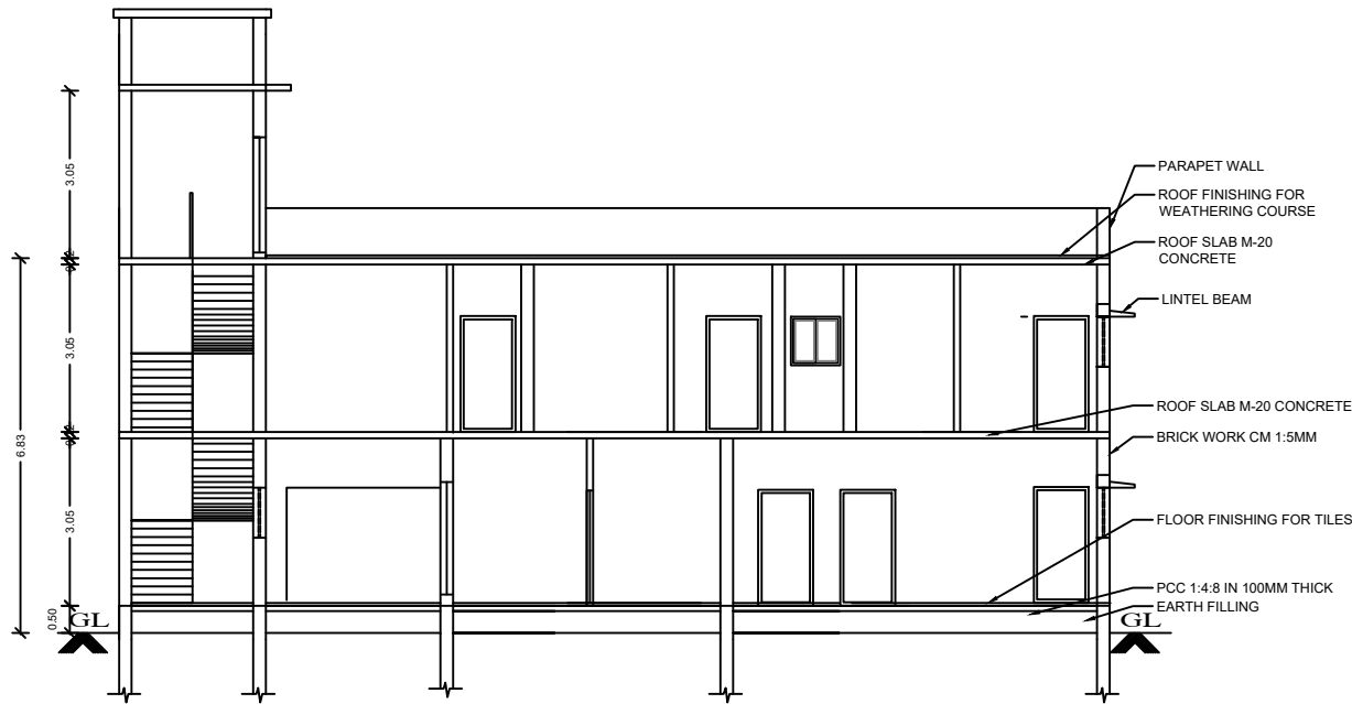
SECTION
