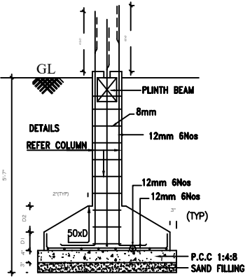
FOUNDATION DETAILS
