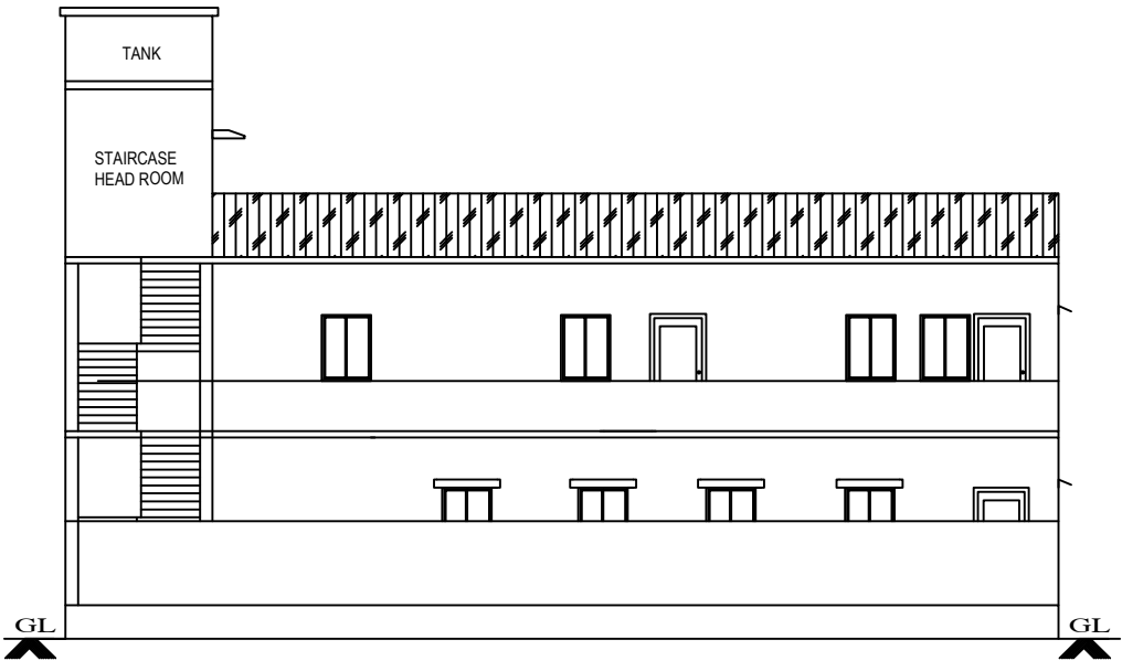
FRONT ELEVATION
