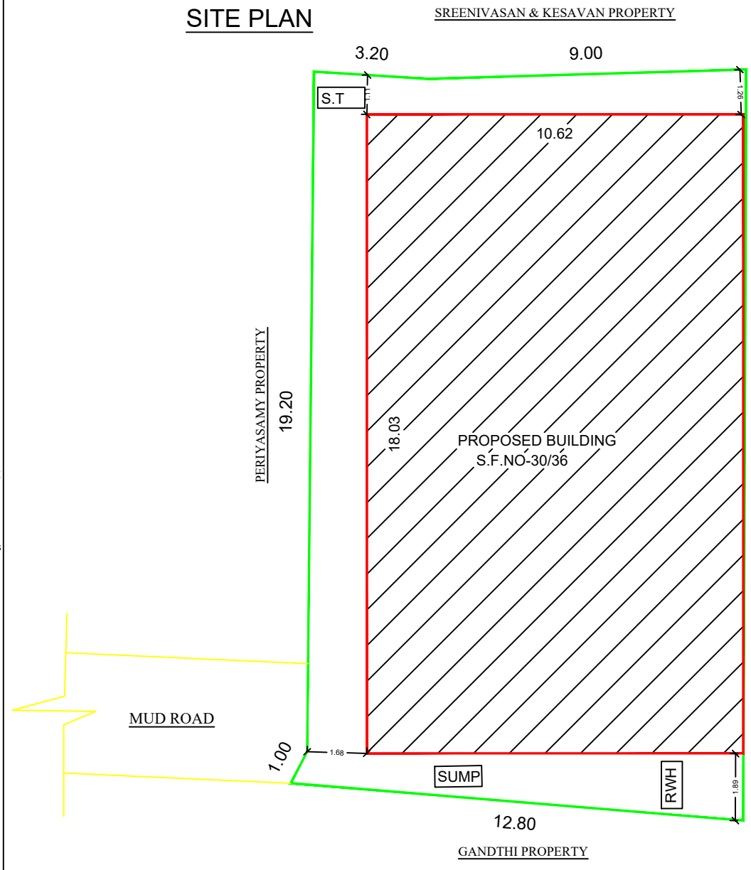
SITE PLAN
