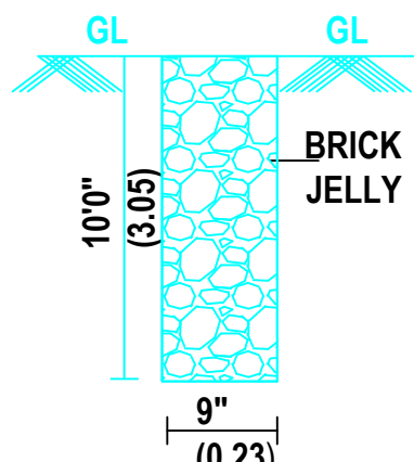
PERCOLATION PIT
