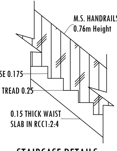
STAIRCASE DETAILS
