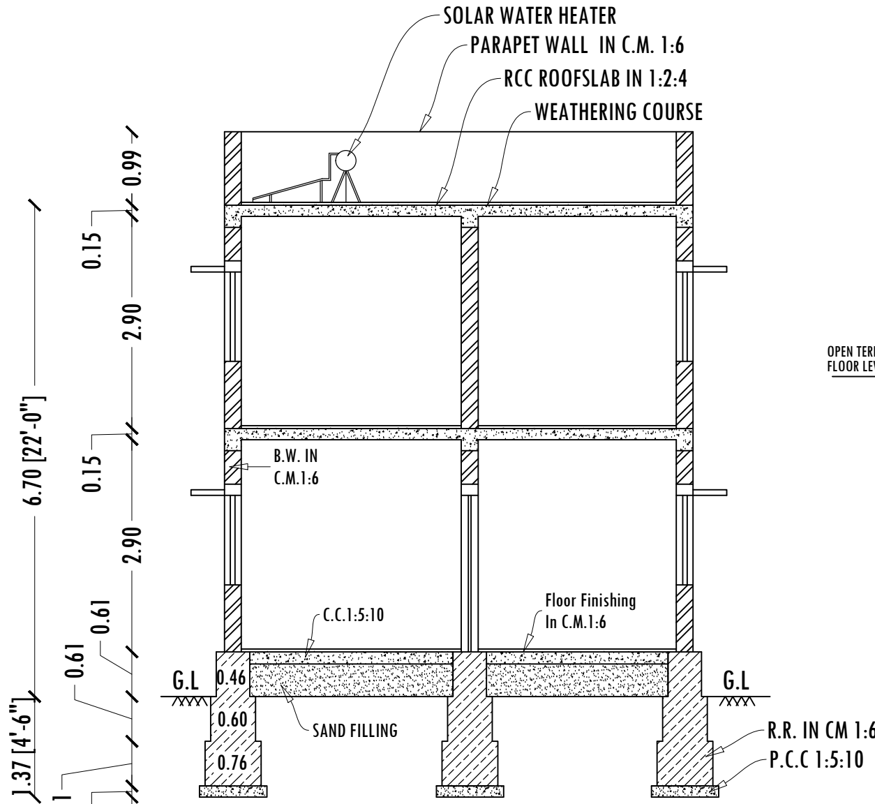
SECTION -AA
