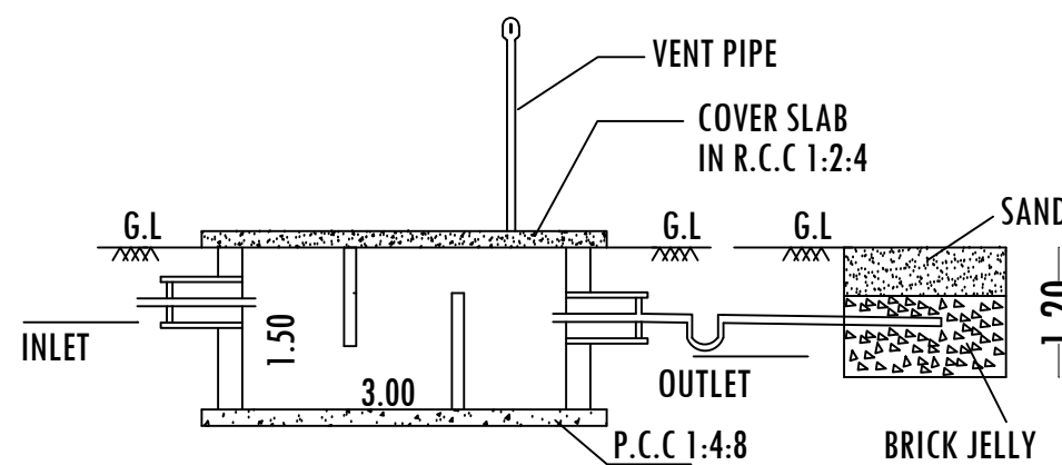
SECTION-AB
