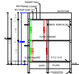
SECTION "A-B"
