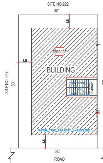
SITE PLAN SCALE:1:100
