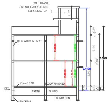
SECTION "A-B"
