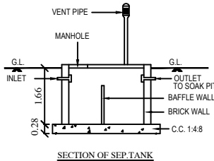
SECTION OF SEPTIC TANK
