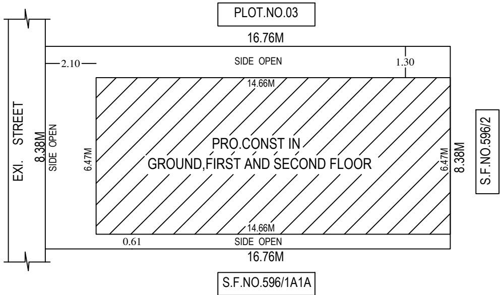
SITE PLAN
