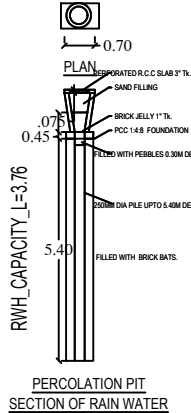
SECTION OF RAIN WATER
