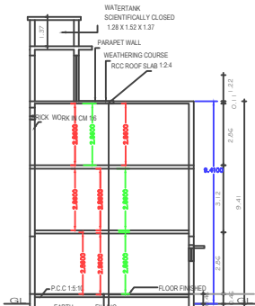
SECTION "A-B"
