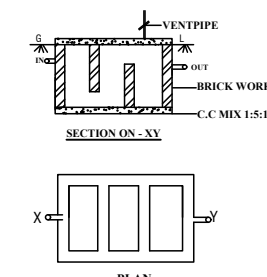
SEPTICTANK DETAILS
