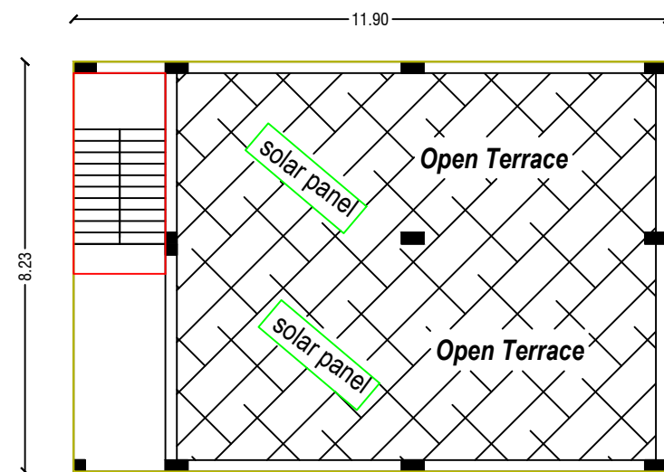
TERRACE SECOND FLOOR PLAN
