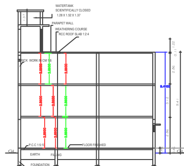
SECTION "A-B"
