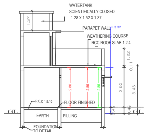
SECTION "A-B"
