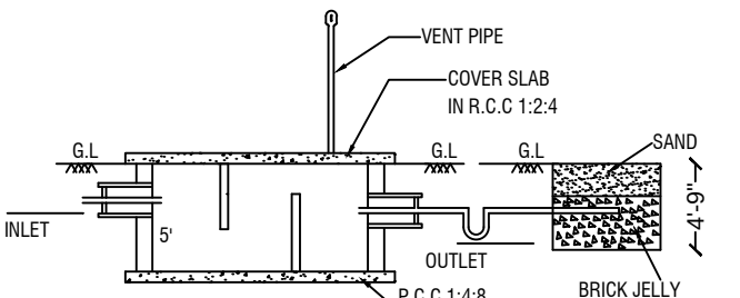
SECTION-AB
