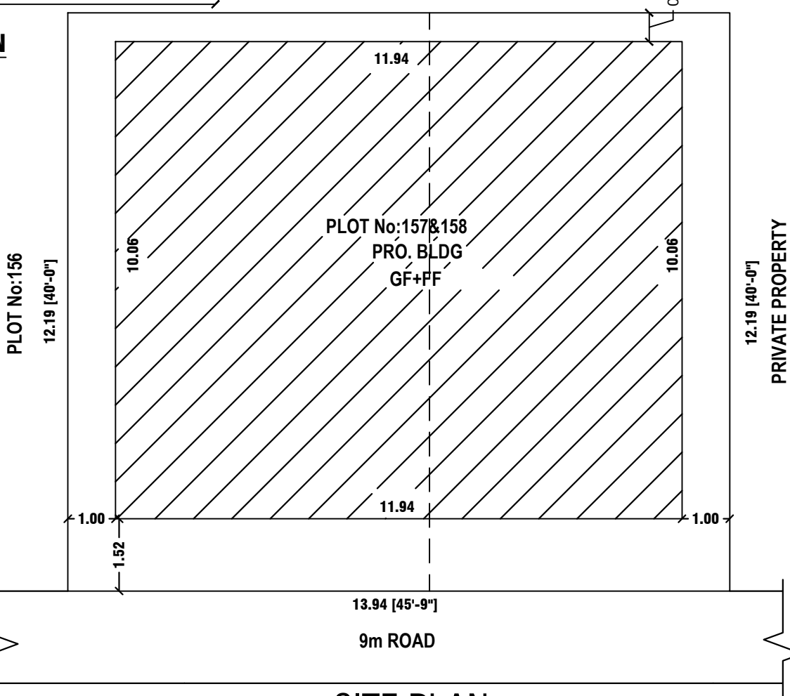
SITE PLAN
