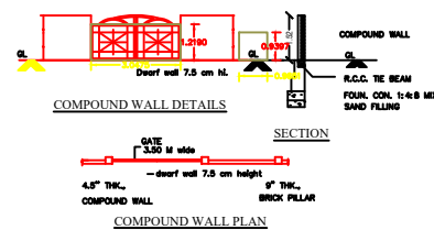
COMPOUND WALL PLAN
