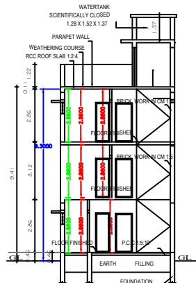
SECTION "A-B"
