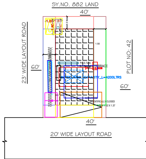
SITE PLAN
