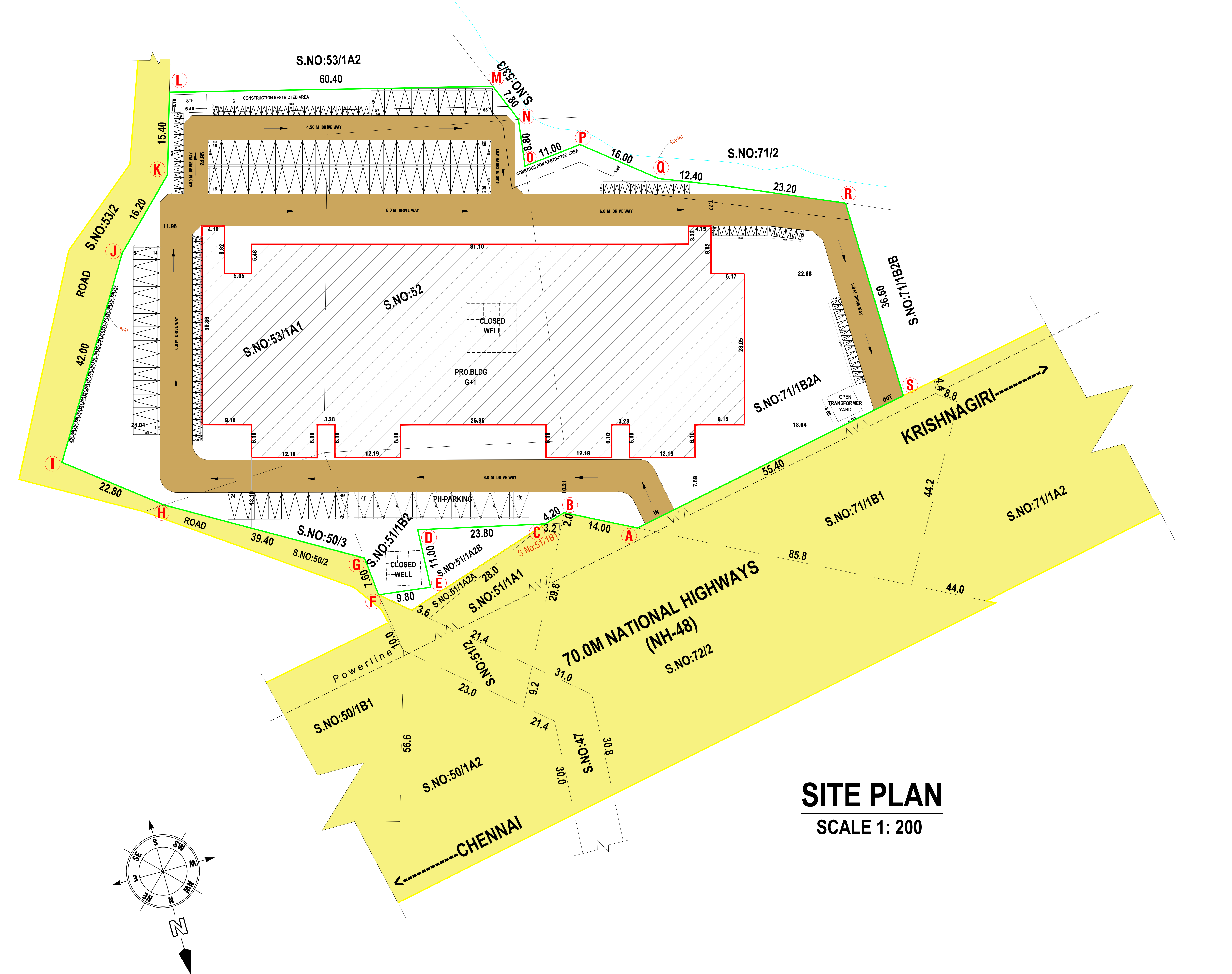
PLAN SHOWING THE PROPOSED CONSTRUCTION OF GROUND , FIRST FLOOR COMMERCIAL BUILDING IN S.NO:50/3 , 51/B2 , 52 , 53/1A1 , 71/1B2A , B.R.G.MADEPALLI VILLAGE & PANCHAYAT , BARGUR UNION , BARGUR TALUK, KRISHNAGIRI DISTRICT.
