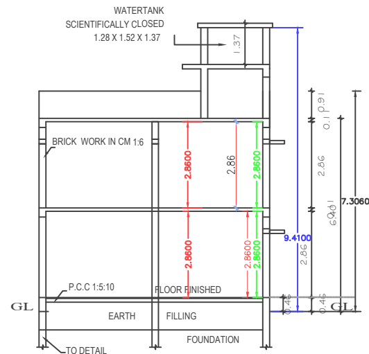
SECTION "A-B"
