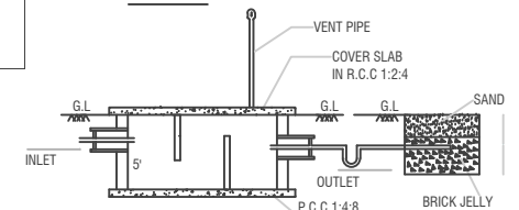
SECTION-AB
