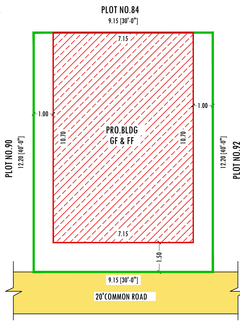
SITE PLAN
