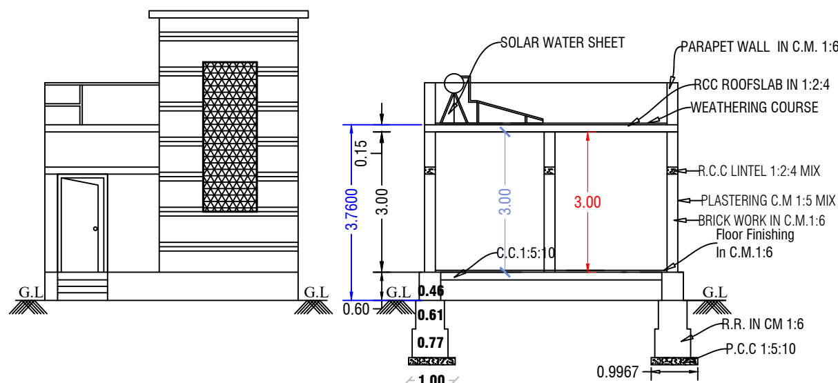
Elevation Plan
