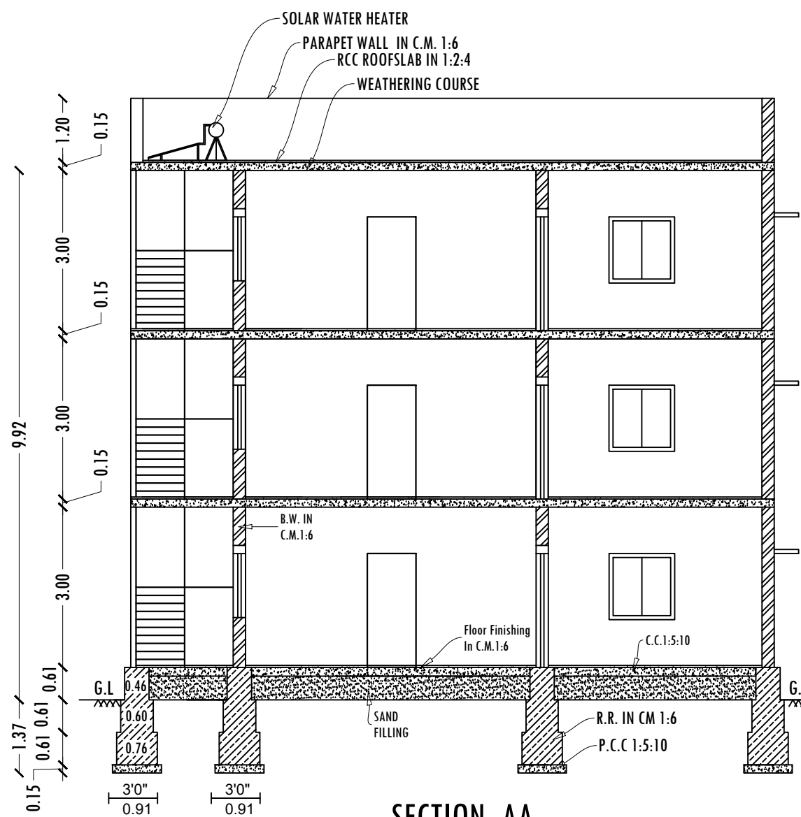
SECTION-AA
