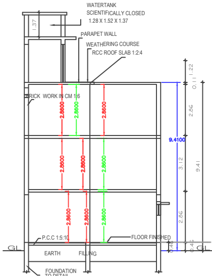
SECTION "A-B"
