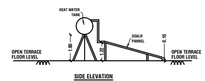
SIDE ELEVATION
