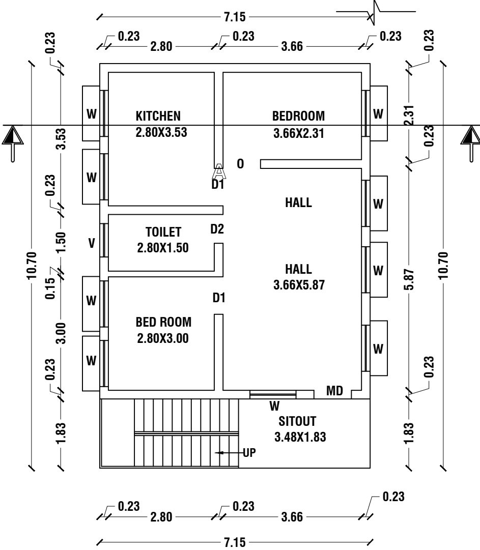
PLAN
