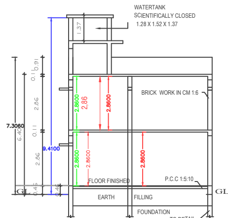
SECTION "A-B"
