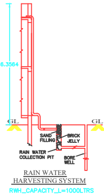
PERCOLATION PIT
