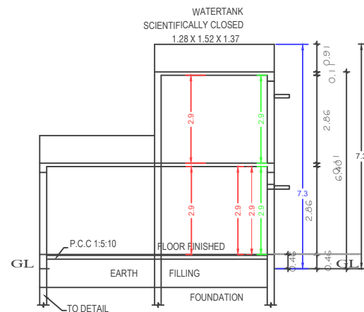
SECTION "A-B"
