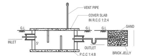
SECTION-AB
