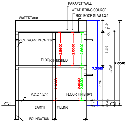
SECTION "A-B"
