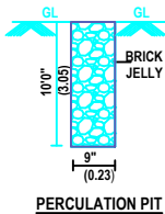
PERCOLATION PIT
