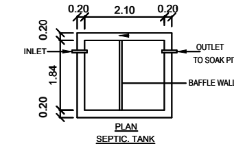
PLAN SEPTIC TANK
