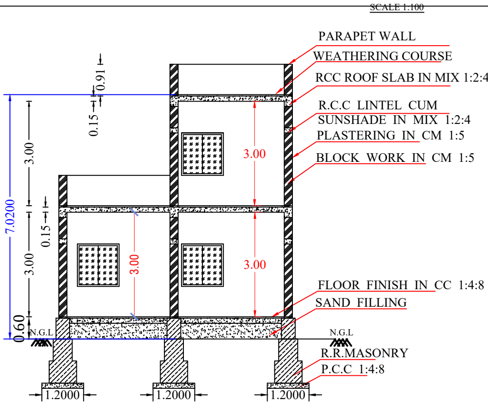
SECTION ON-'AB'
